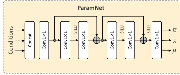
Fig. 3. Structure of ParamNet. The parameter of logistic mixture model \pi, \mu , and s is generated by ParamNet.
