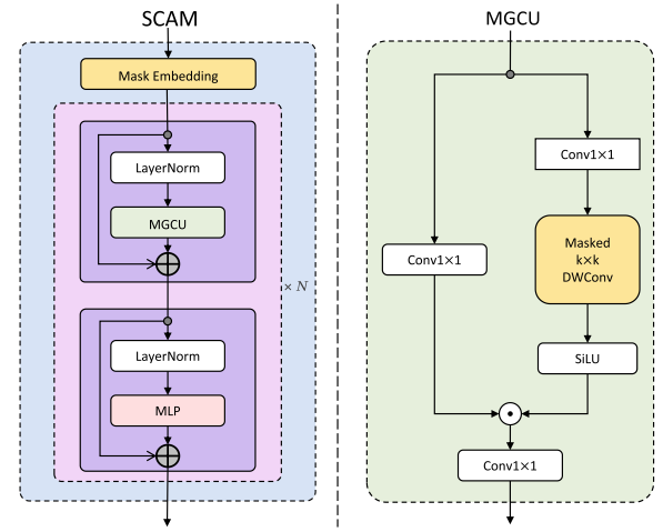
Fig. 4. Architecture of SCAM and its internal MGCU block. SCAM aggregates spatial context under causality constraints using stacked MGCUs, each combining masked depthwise convolution with gated feature mixing.
