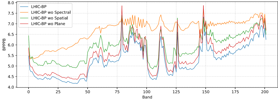
Fig. 10. Band-wise compression performance comparison in terms of bpppb on HyspecNet-11K.
