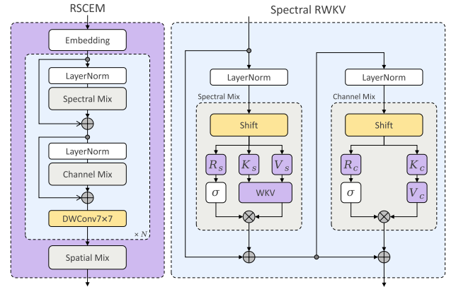
Fig. 6. Architecture of the RSCEM, integrating spectral, channel, and spatial mix blocks. The right panel expands the RWKV-based mixers, where shift and WKV operations capture long-range dependencies with linear complexity.
