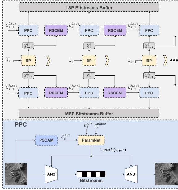
Fig. 8. Streaming coding scheme during inference mode for the proposed LHIC-BP, where PPC denotes the combination of PSCAM, ParamNet, and ANS coding.
